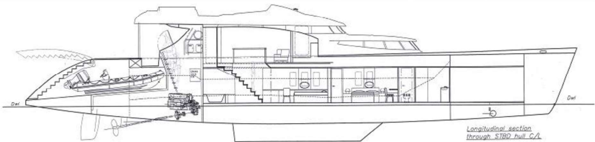
Longitudinal section through vessel C/L
