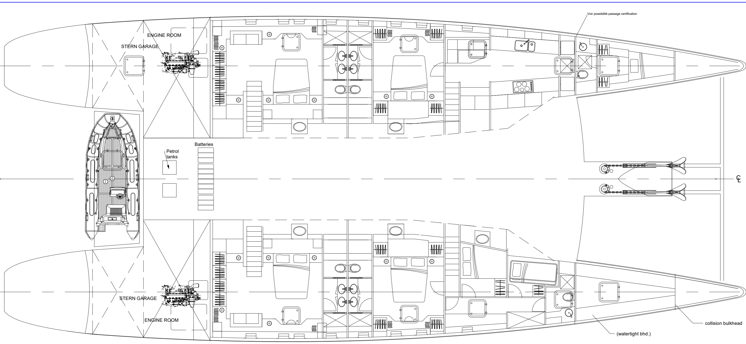
Plan view - lower deck
